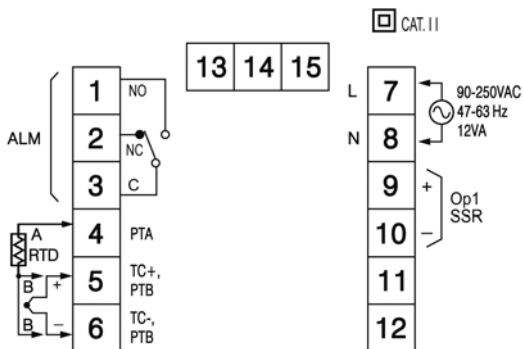
Figure 2.6 Rear Terminal Connection
